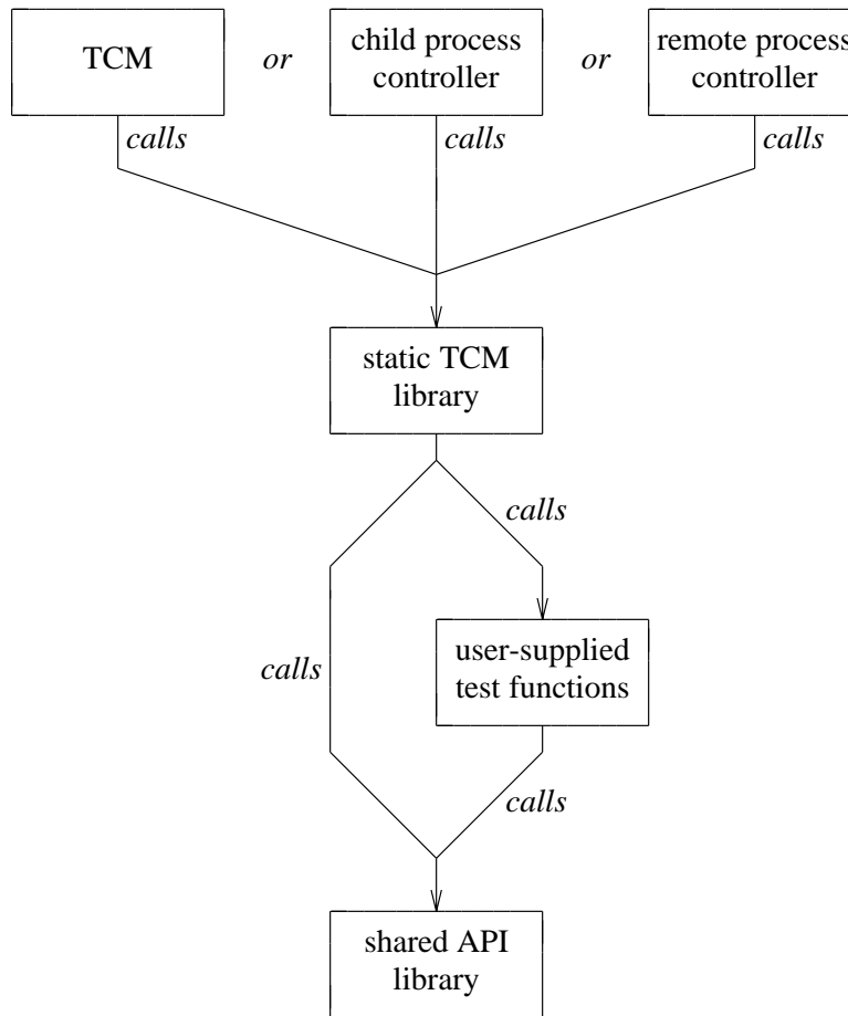
Figure 21. Relationship between the API components and the user-supplied code when a shared API library is used
